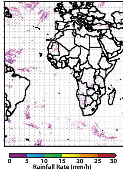
Example of the Rainfall Rate product as generated by the GOES-R Rainfall Rate algorithm using Meteosat-8/SEVIRI (Spinning Enhanced Visible and Infrared Imager) data on January 7, 2005 12:45 UTC. Credit: NOAA/NESDIS/STAR
